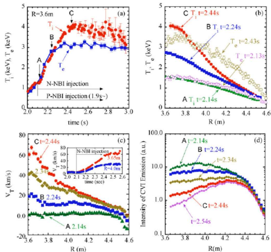
Fig. 1. (a) Evolutions of central ion temperature and electron temperature and radial profiles of (b) ion temperature and electron temperature, (c) toroidal flow velocity, and (d) intensity of the C VI emission in the high-ion temperature discharge.
